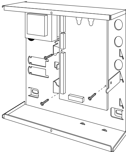
Figure 6. Installation du coffret
