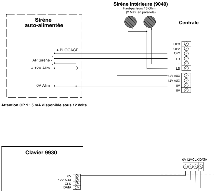
Figure 11. Centrale 9750 - Raccordements sirène et clavier
